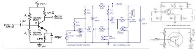
Circuit
